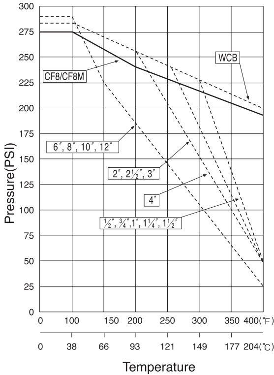
10K-Class 150 - 2 piece Design PTFE Seats
