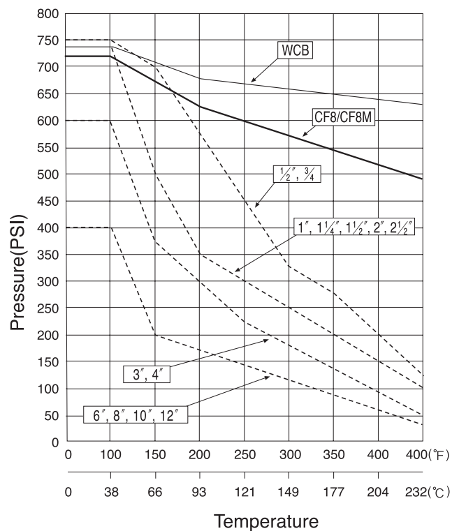
20K-Class 300 - 2 piece Design Glass or Carbon Reinforced PTFE Seats
