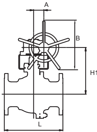
Size 6" (150) to 8" (200) Gear Operated (Option)
