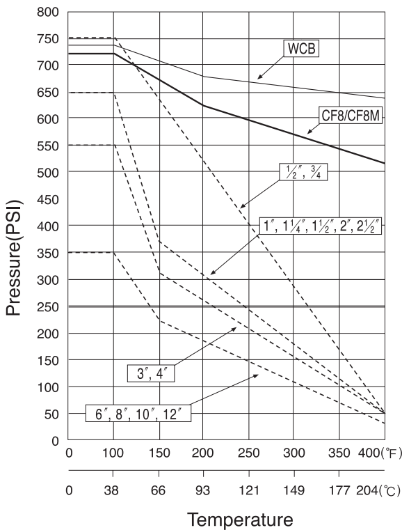
20K-Class 300 - 2 piece Design PTFE Seats
