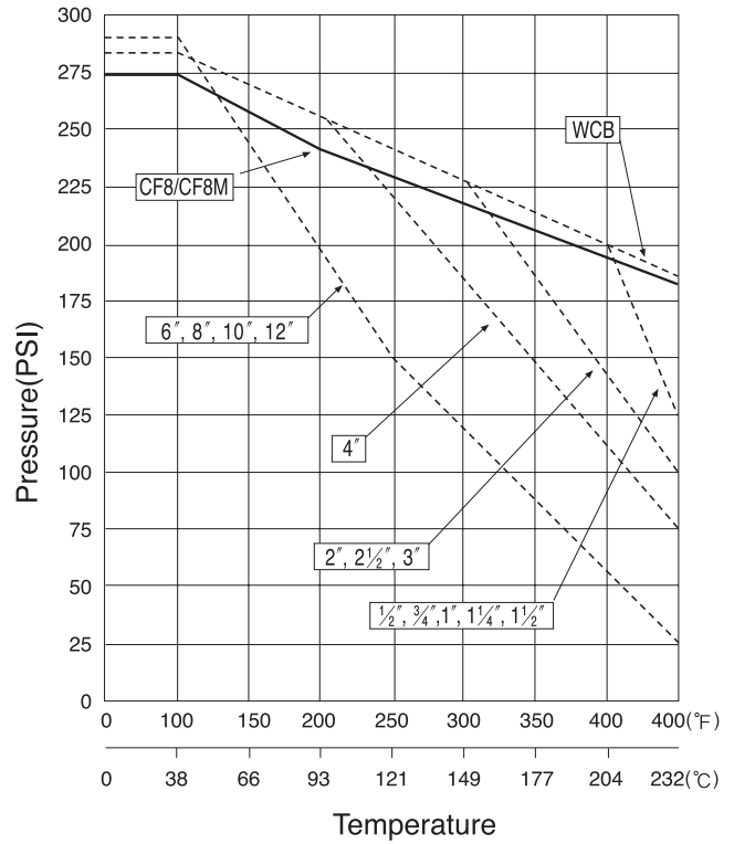
10K-Class 150 - 2 piece Design Glass or Carbon Reinforced PTFE Seats
